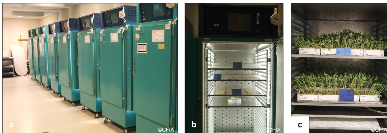
Figure 8.5. 'Dry' germination cabinets: a in germination room; b with door open and showing probes; c with soybean seedlings (images courtesy of ISTA accredited laboratory CA08)
