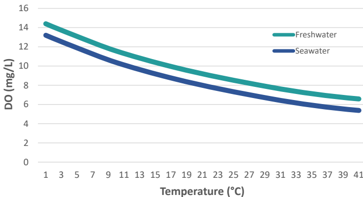
Figure 5.6 Concentration in mg/L at 100% saturation of dissolved oxygen (DO) in fresh water and in saltwater
