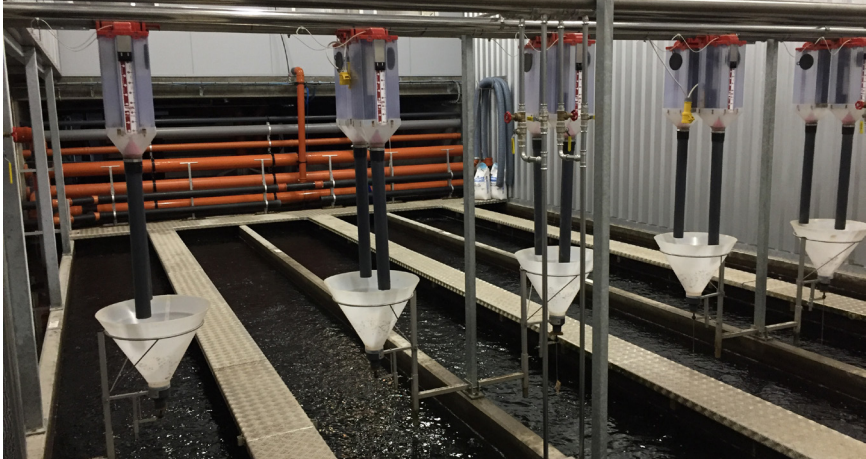
Figure 5.9 An example of an automated feeding system
