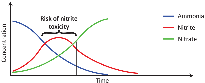
Figure 5.3 Fluctuations in the concentration of different nitrogen compounds when starting up and maturing a biofilter
