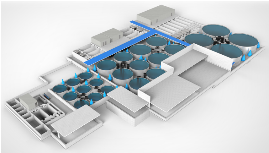
Figure 1.4 A modern RAS split into different modules to make the system design match the specific needs of fish at different growth stages
