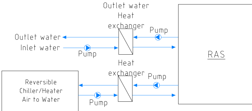
Figure 2.19 Schematic illustration of the water temperature regulation in a RAS
