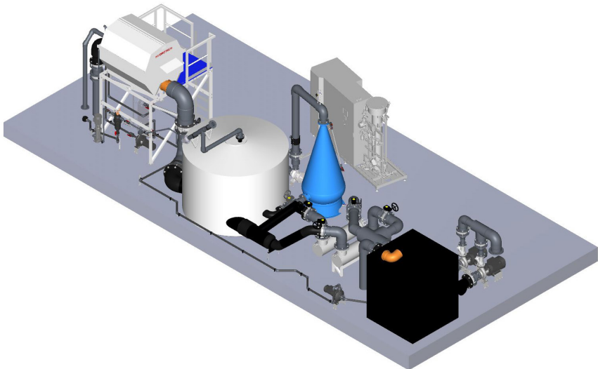
Figure 2.25 Example of intake water disinfection for treatment before use in the RAS
