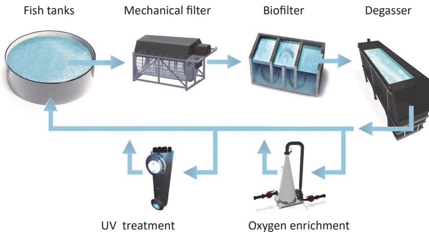
Figure 2.1 Principle drawing of a recirculation system
