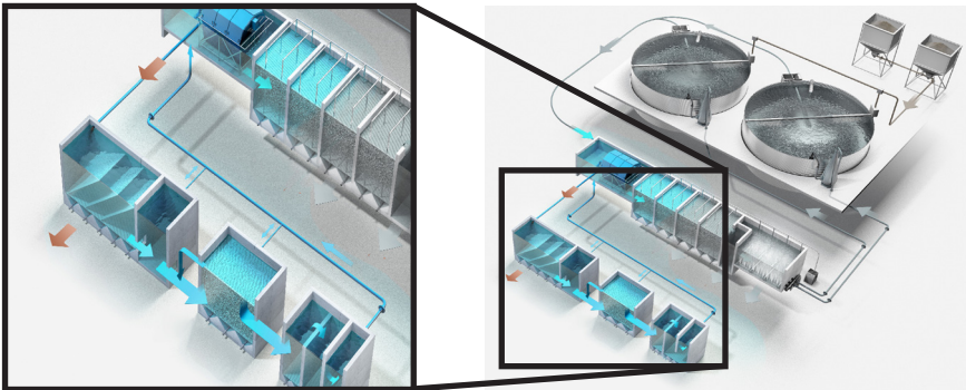
Figure 6.8 Denitrification loop in a RAS taking the sludge water from the mechanical filter through a settling system before it enters a denitrification chamber
