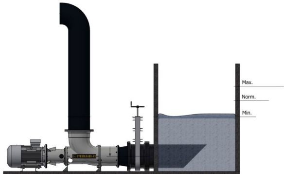
Figure 2.22 Example of dry set-up for a main water pump
