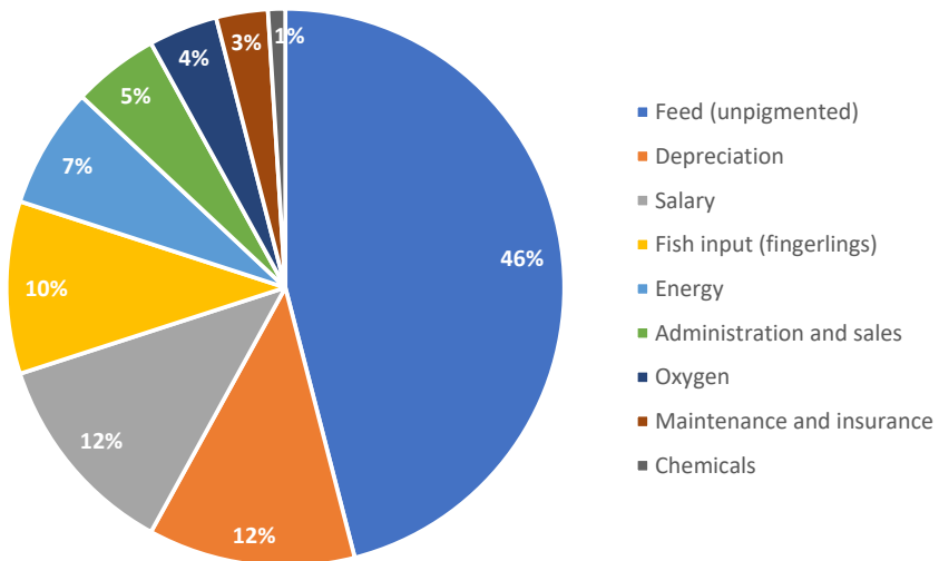
Figure 4.4 Example of cost distribution for a single RAS production unit for portion sized trout (2 000 tonnes/year) taking in fingerlings and growing them to 300–500 g
