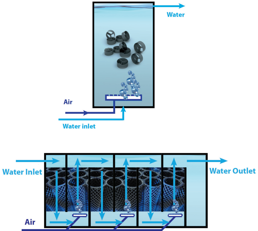
Figure 2.9 Moving bed (top) and fixed bed biofilters (bottom)
