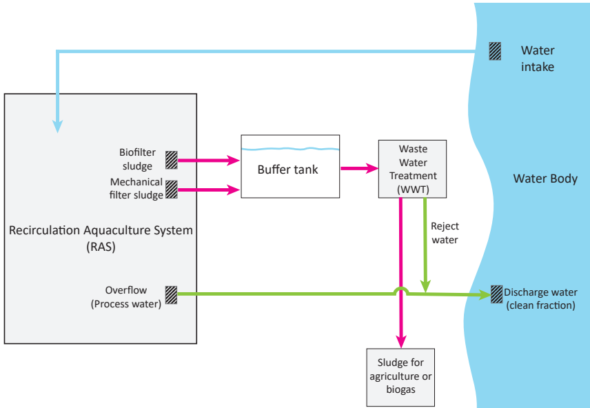
Figure 6.2 A sketch of flows to and from a recirculation aquaculture system
