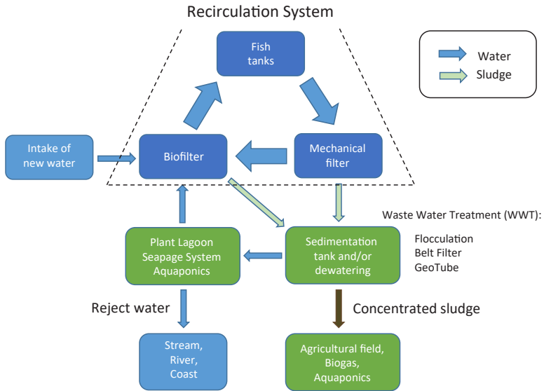
Figure 6.3 The pathways of sludge and water inside and outside a recirculation system
