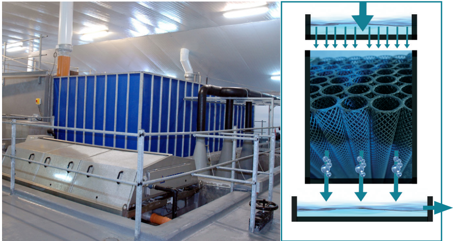
Figure 2.11 Photo and drawing of a trickling filter wrapped in a blue plastic liner to eliminate splashing on the floor
