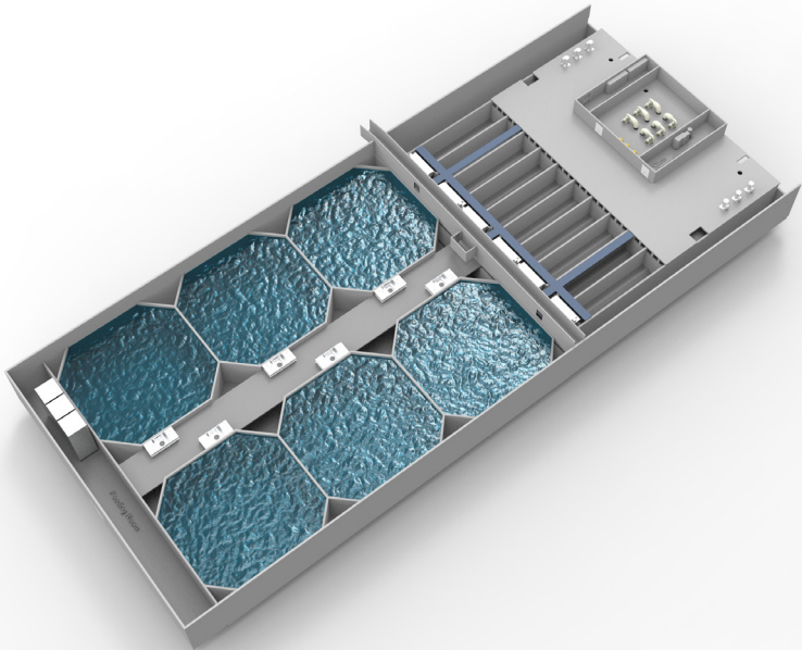
Figure 2.3 An example of octagonal tank design in a recirculation system saving space yet achieving the good hydraulic effects of the circular tank
