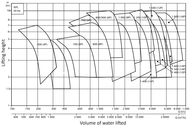
Figure 2.20 Lifting pumps type KPL for efficient lifting of large amounts of water
