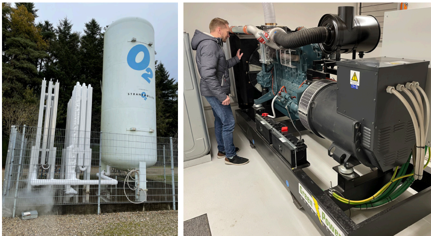
Figure 2.24 Liquid oxygen (LOX) tank and an electrical emergency generator driven by diesel
