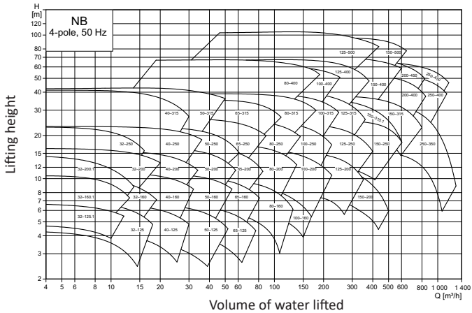
Figure 2.21 Centrifugal pumps type NB for pumping water when high pressure or high lifting heights are needed
