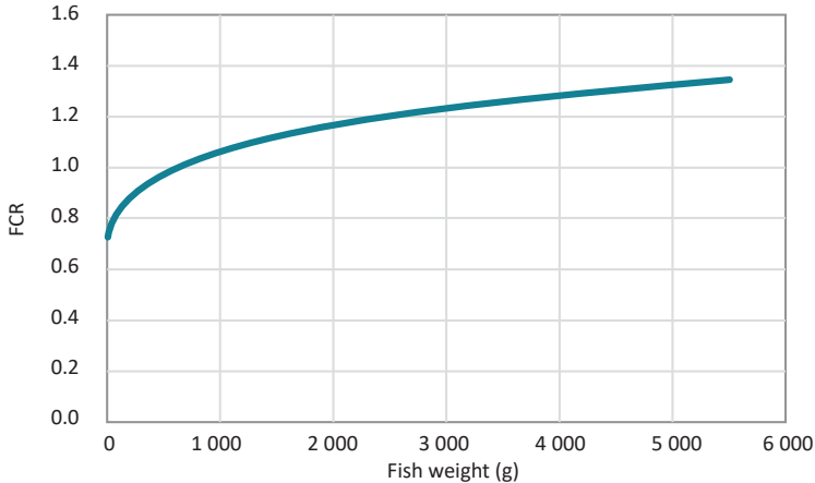
Figure 3.2 Example of feed conversion rate (FCR) of Atlantic salmon in a RAS related to fish weight at 14 °C
