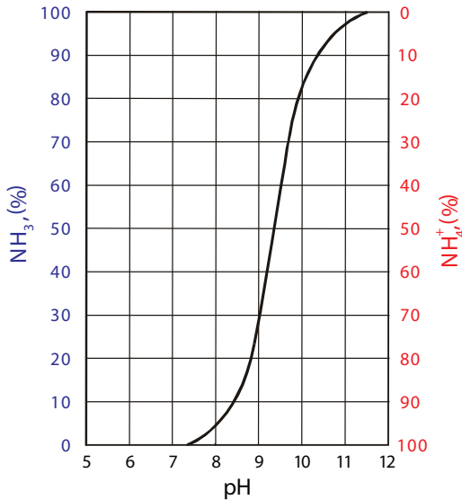
Figure 2.6 The equilibrium between ammonia ( \text{NH}_3 ) and ammonium ( \text{NH}_4^+ ) at 20 °C.
