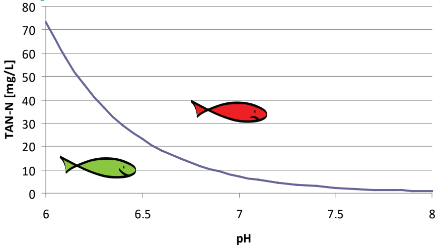
Figure 2.7 The relation between measured pH and the amount of TAN available for breakdown in the biofilter, based upon a toxic ammonia concentration of 0.02 mg/L at 15 °C
