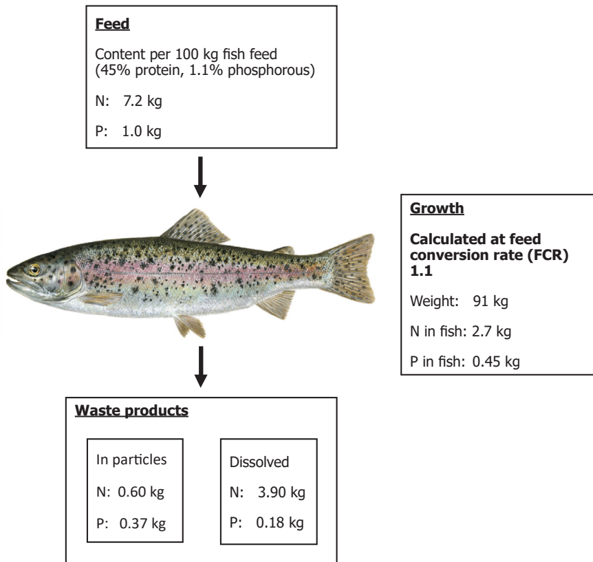
Figure 6.1 Excretion of nitrogen (N) and phosphorus (P) from farmed fish. Note the large amount of N excreted as dissolved matter
