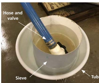
Collecting larvae in sieve
