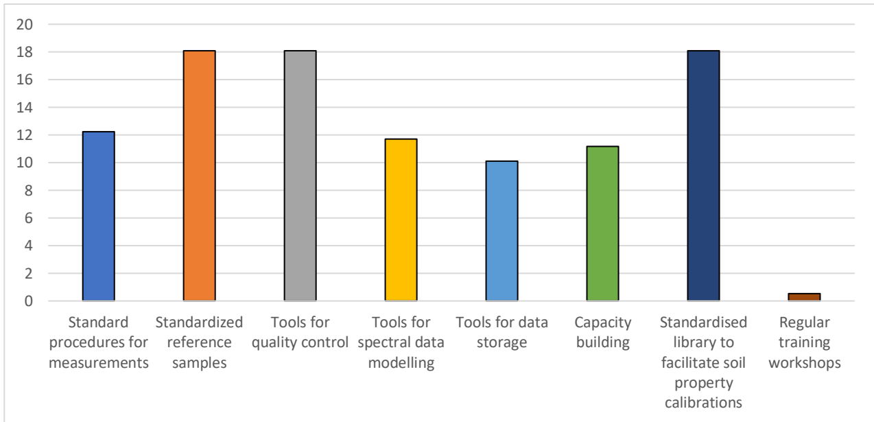
Figure 17 – Laboratories main requirements to improve their spectral measurements, expressed in percentages of the total answers to the survey.
